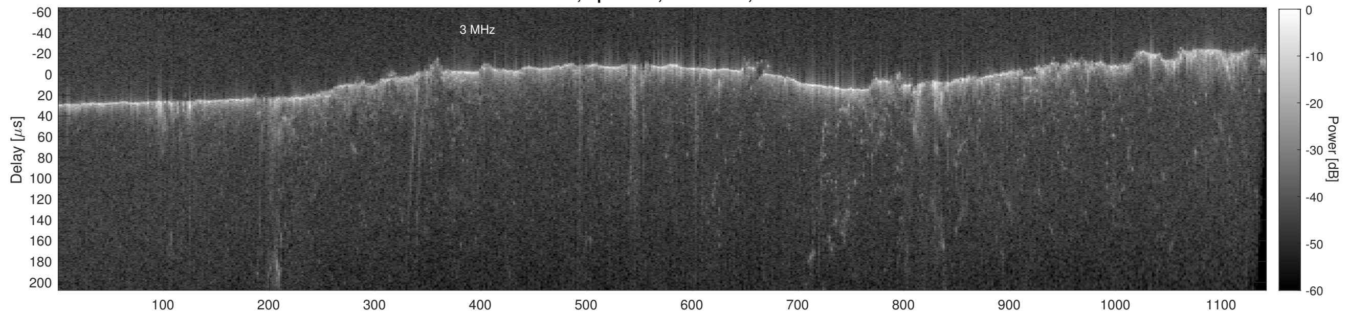
Orbit 11240, Cluttergram
