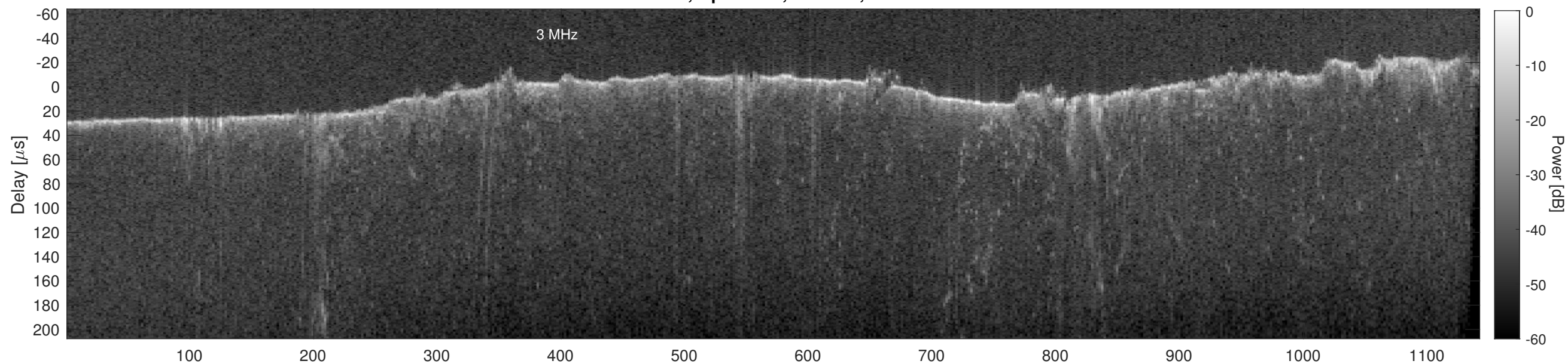
Orbit 11240, Cluttergram
