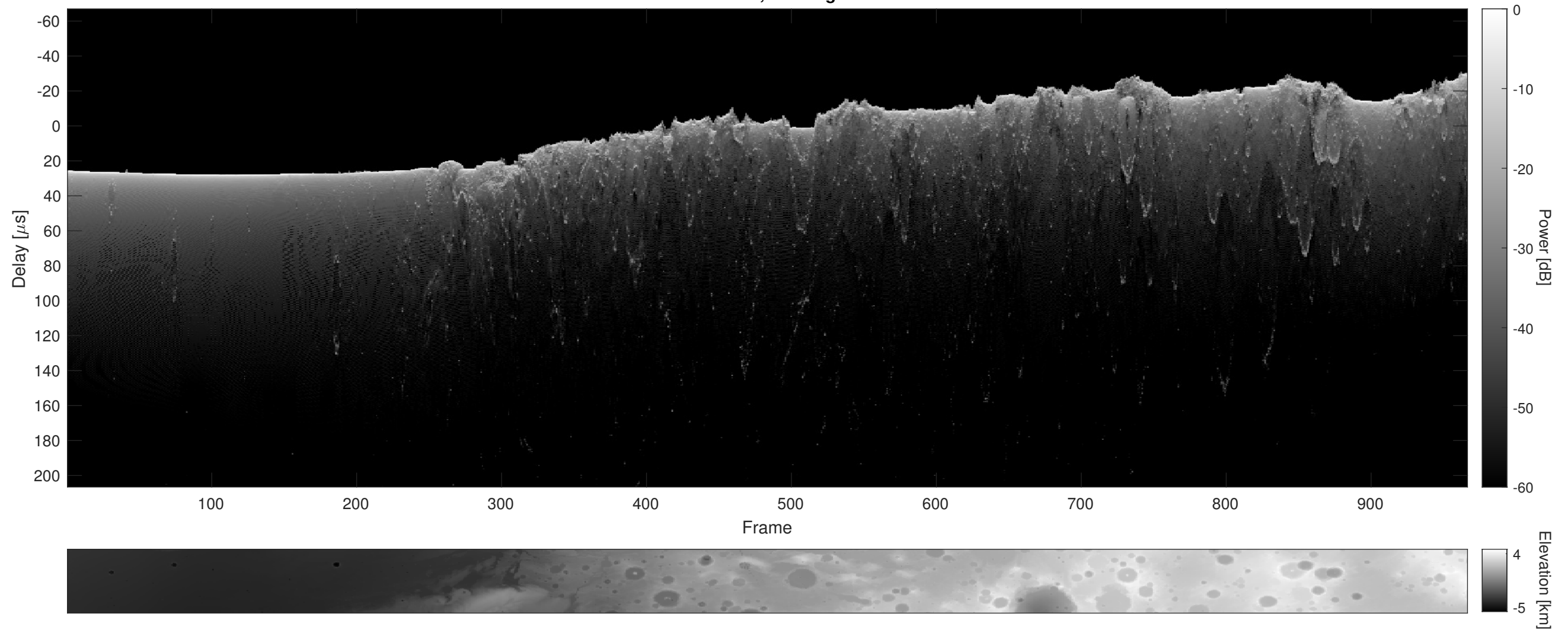
Orbit 11246, Cluttergram
