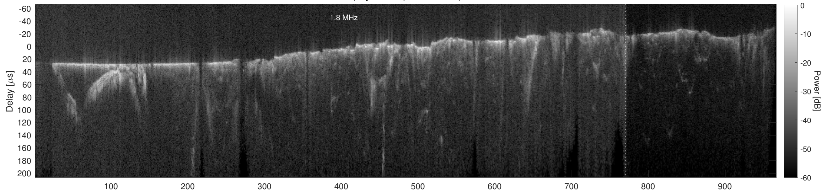
Orbit 11246, Cluttergram
