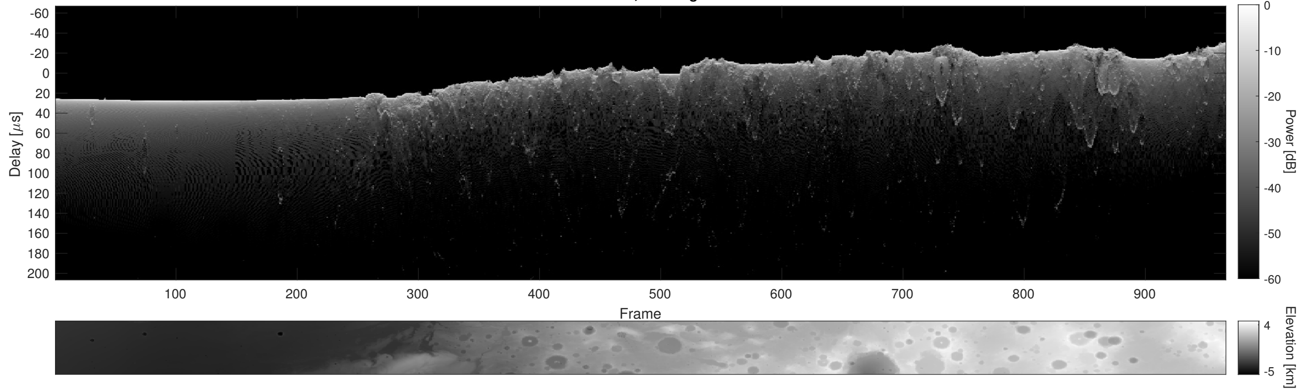
Orbit 11246, Cluttergram
