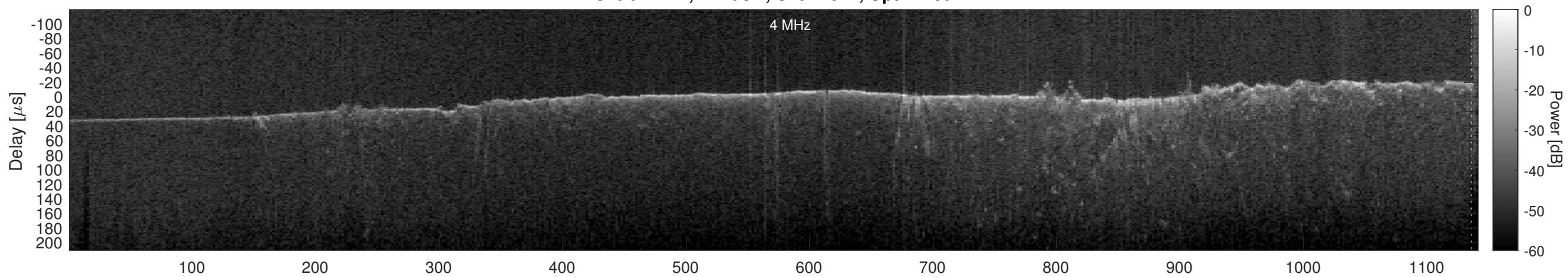
Orbit 11247, Cluttergram
