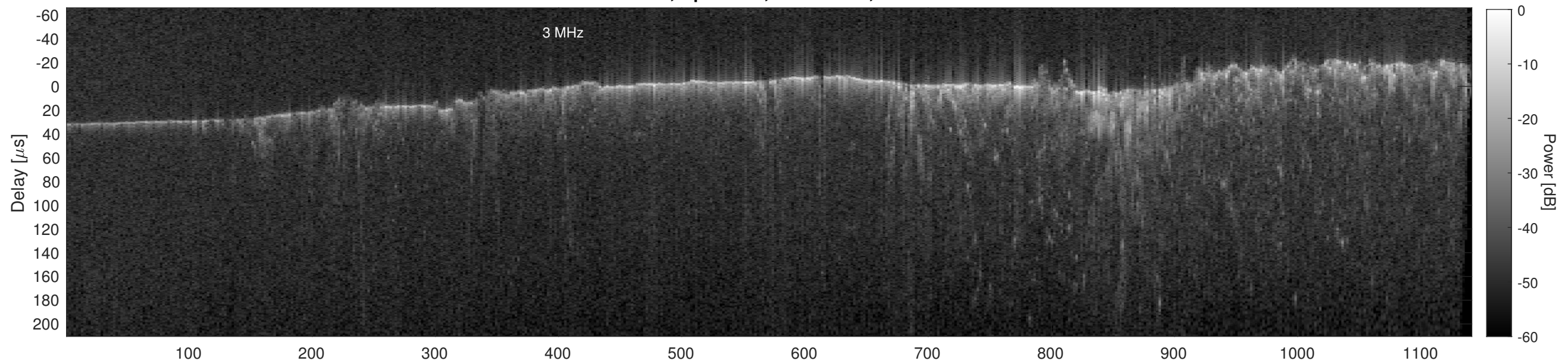
Orbit 11247, Cluttergram
