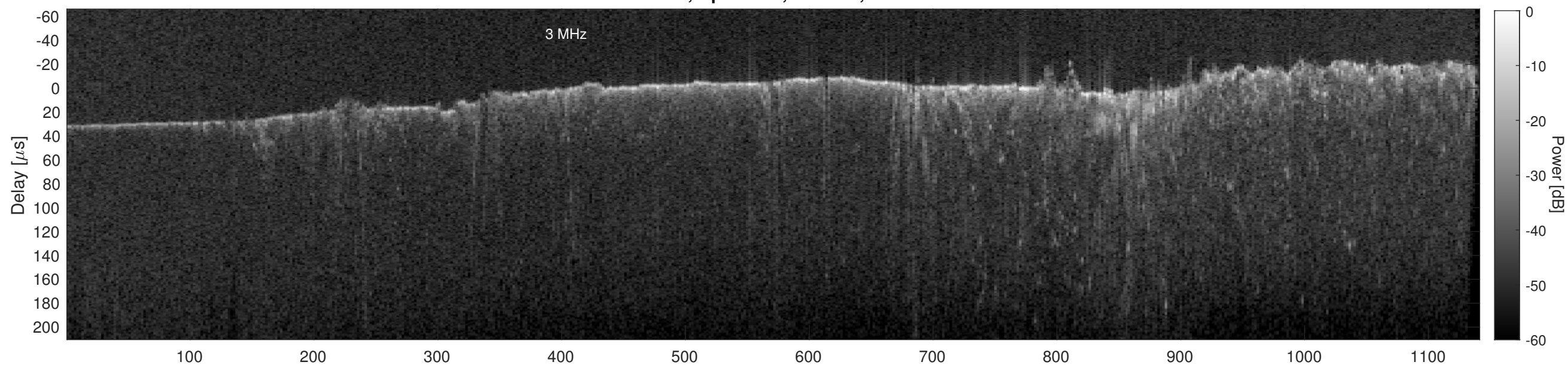
Orbit 11247, Cluttergram
