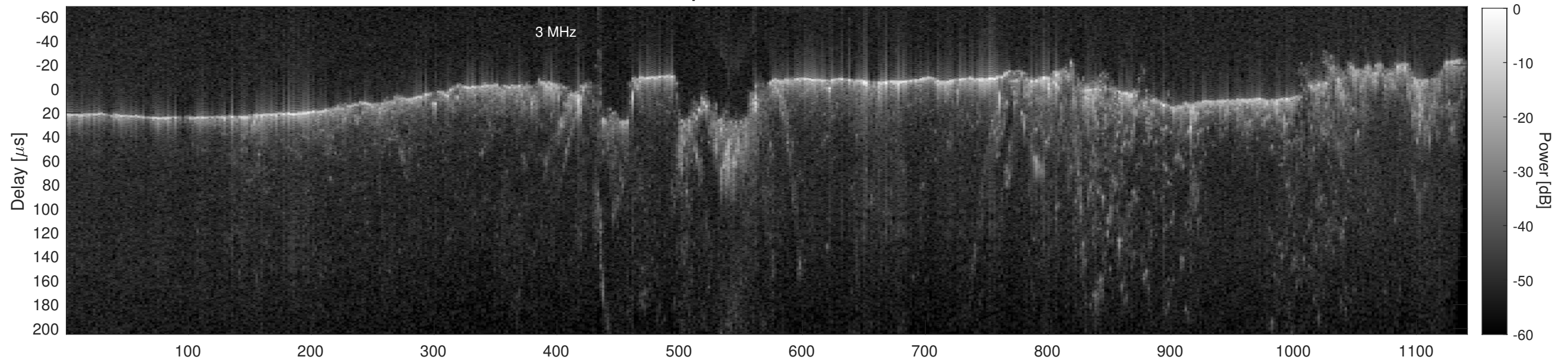
Orbit 11252, Cluttergram
