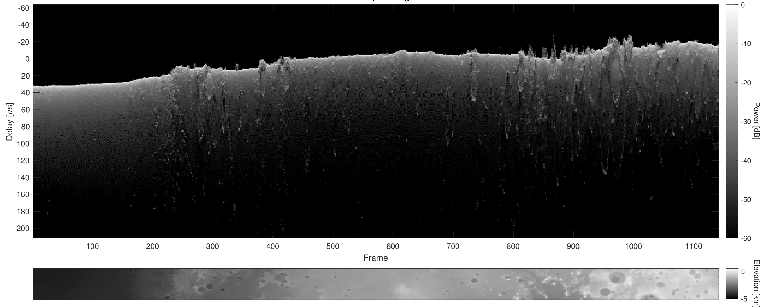
Orbit 11254, Cluttergram
