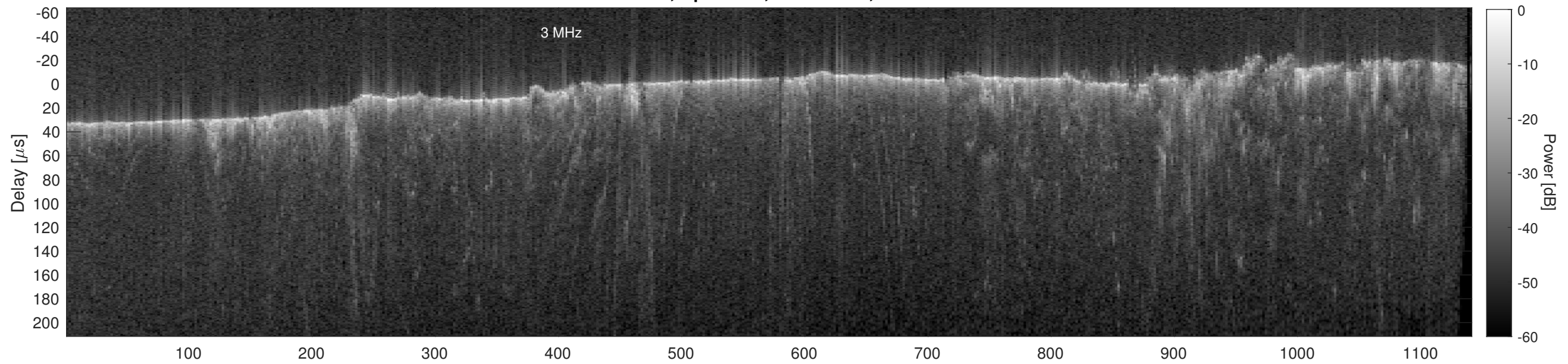
Orbit 11254, Cluttergram
