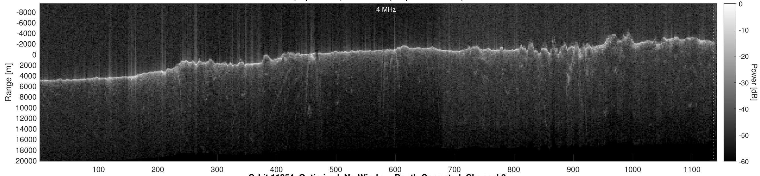
Orbit 11254, Optimized, No Window, Depth-Corrected, Channel 2
