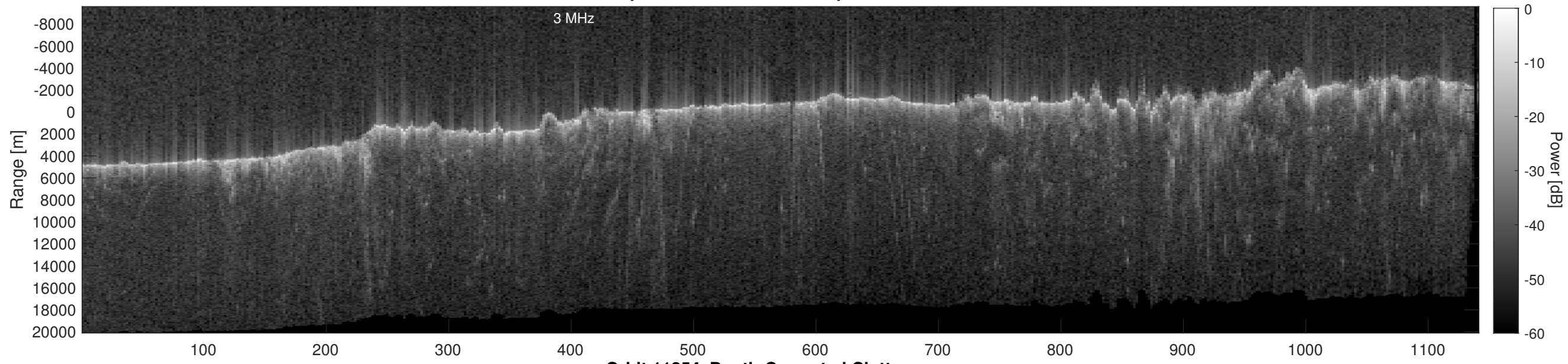
Orbit 11254, Depth-Corrected Cluttergram
