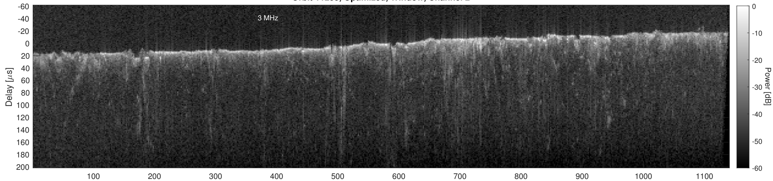
Orbit 11255, Cluttergram
