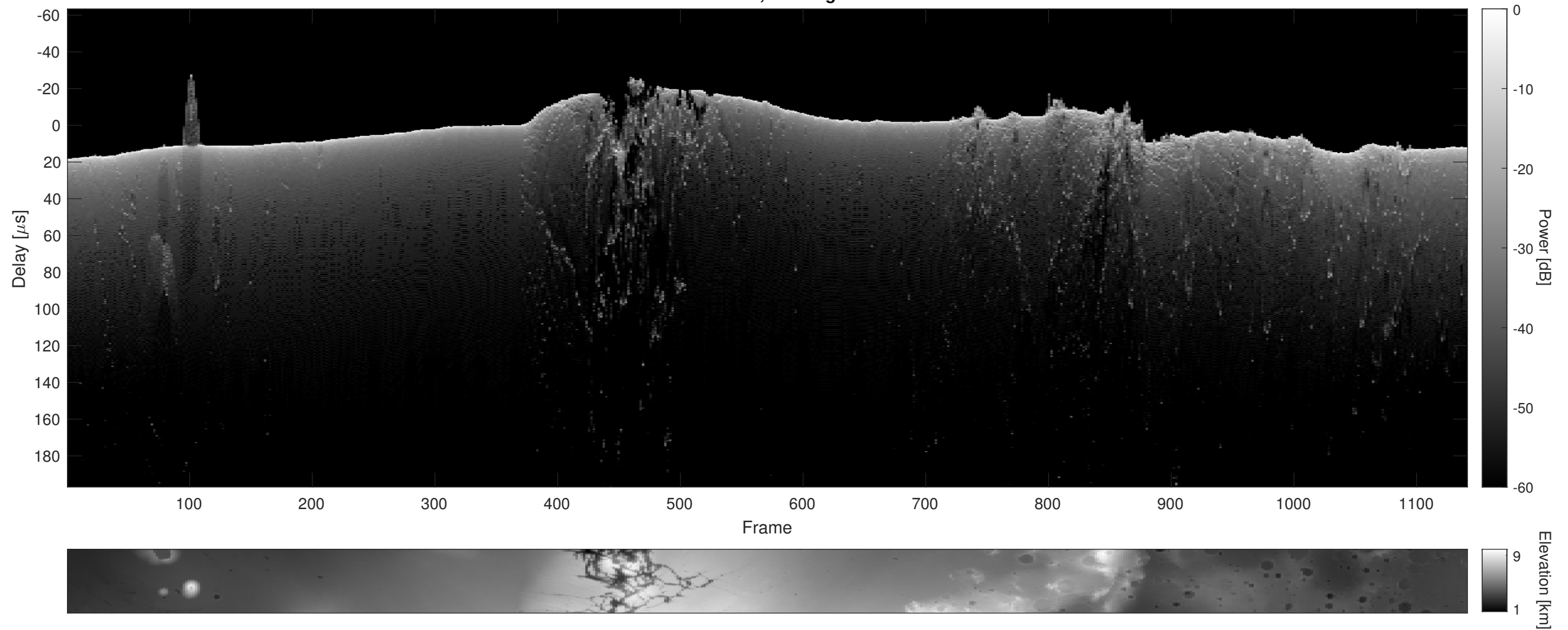
Orbit 11256, Cluttergram
