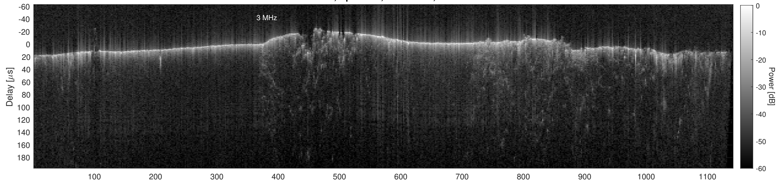
Orbit 11256, Cluttergram
