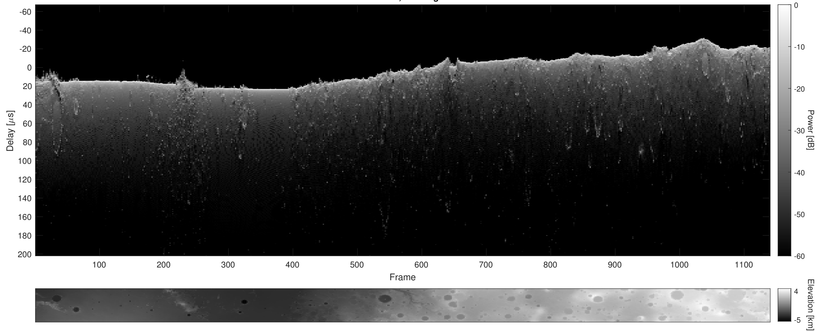
Orbit 11257, Cluttergram
