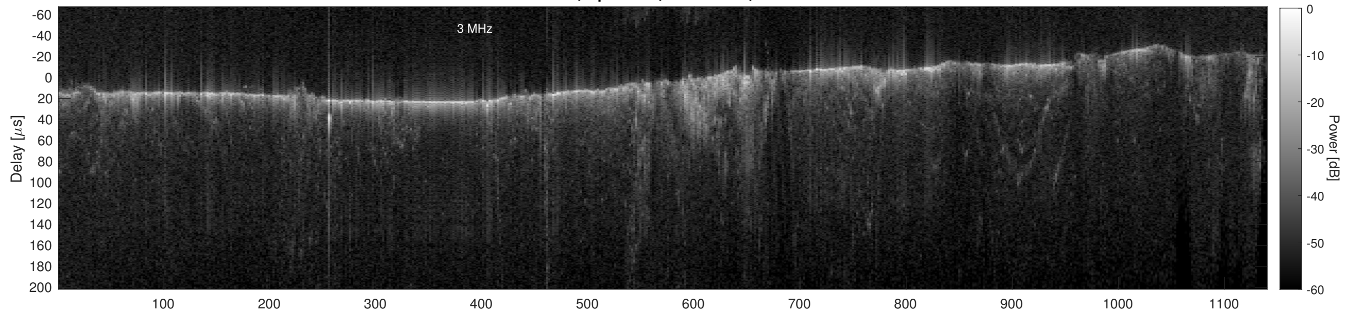
Orbit 11257, Cluttergram
