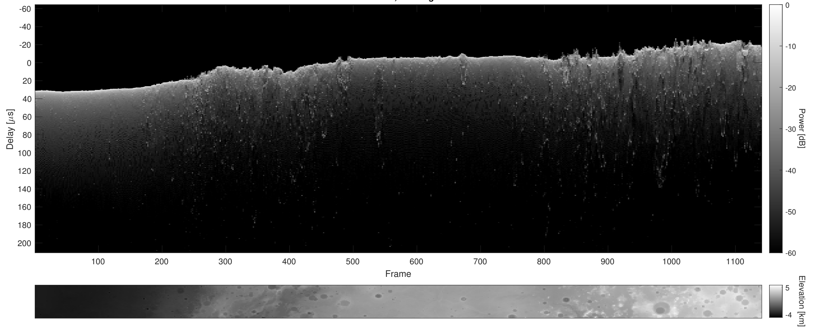
Orbit 11261, Cluttergram
