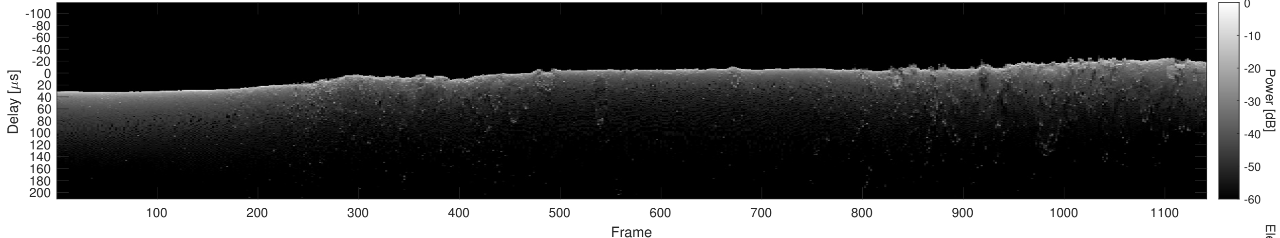
Orbit 11261, Cluttergram
