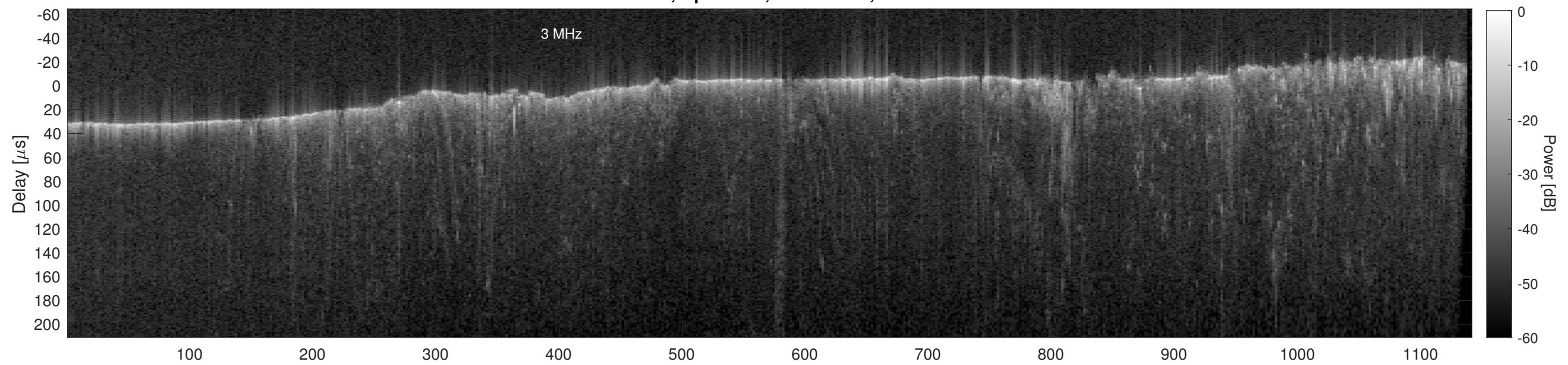
Orbit 11261, Cluttergram
