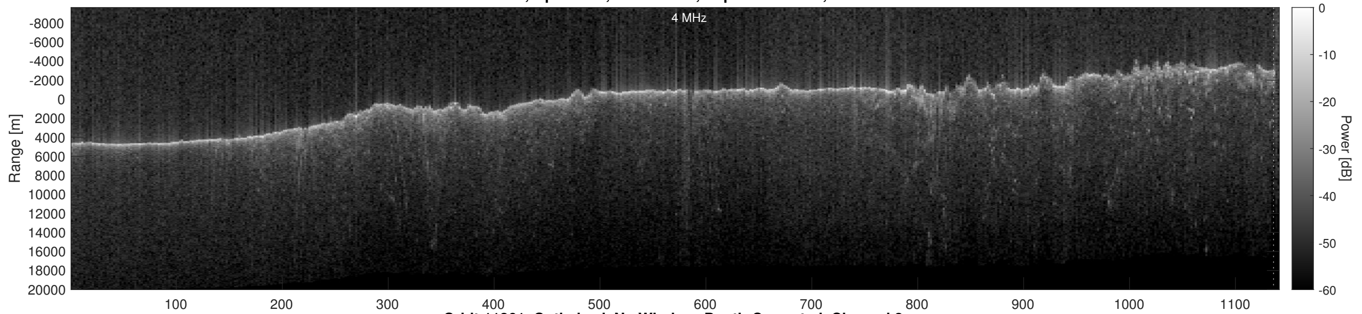
Orbit 11261, Optimized, No Window, Depth-Corrected, Channel 2
