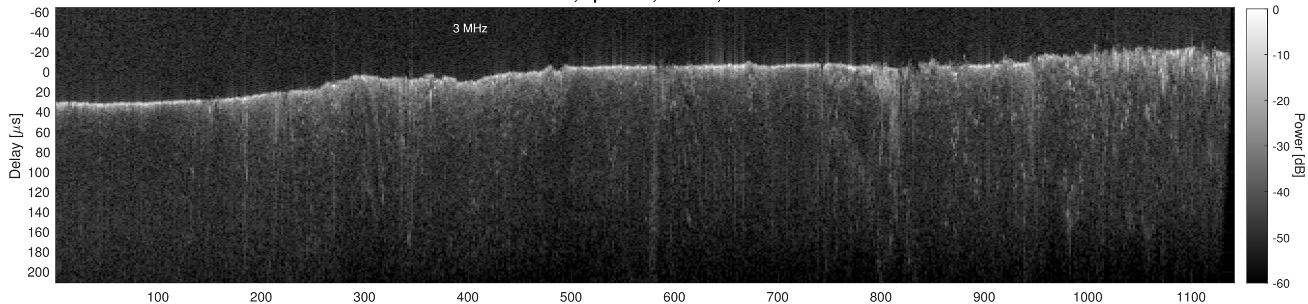
Orbit 11261, Cluttergram
