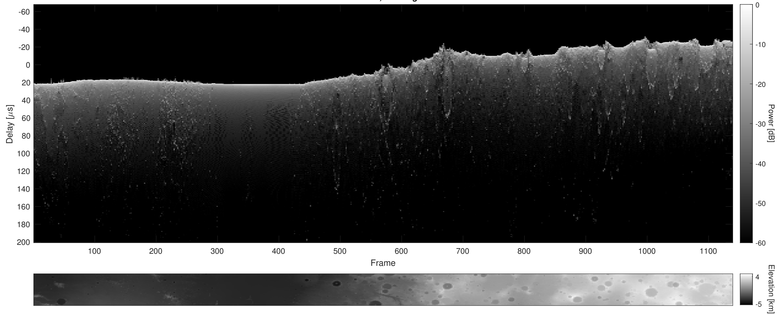
Orbit 11264, Cluttergram
