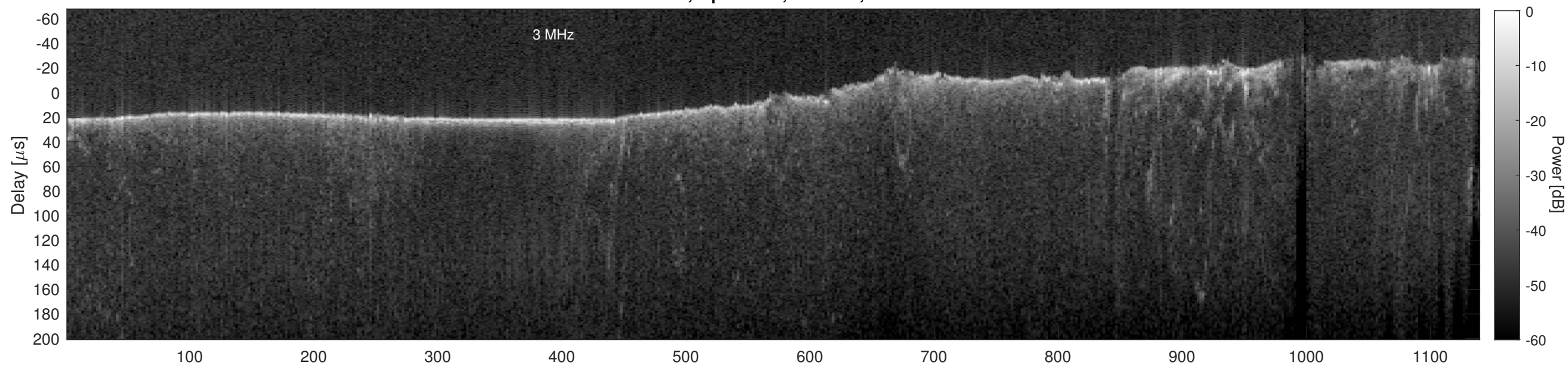
Orbit 11264, Cluttergram
