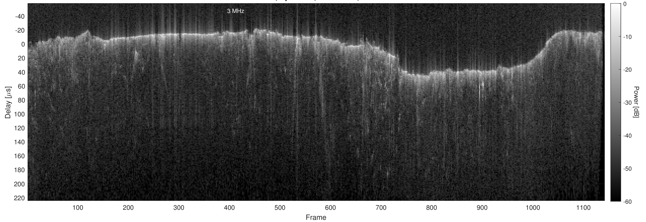
Orbit 11265, Optimized, No Window, Channel 2
