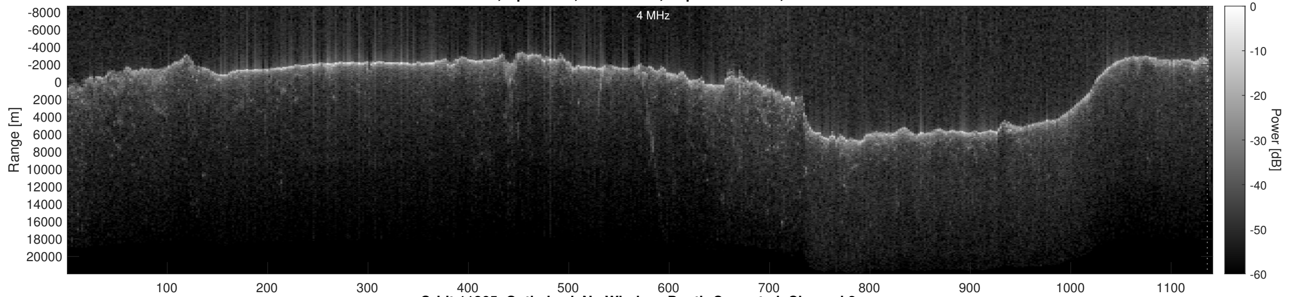
Orbit 11265, Optimized, No Window, Depth-Corrected, Channel 2
