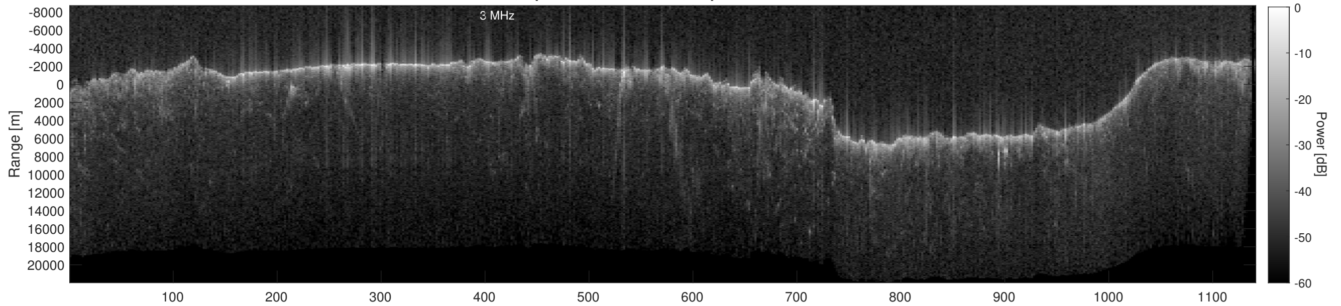
Orbit 11265, Depth-Corrected Cluttergram
