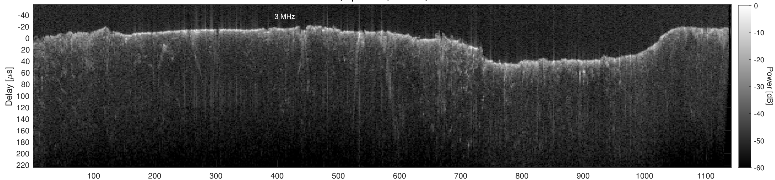
Orbit 11265, Cluttergram
