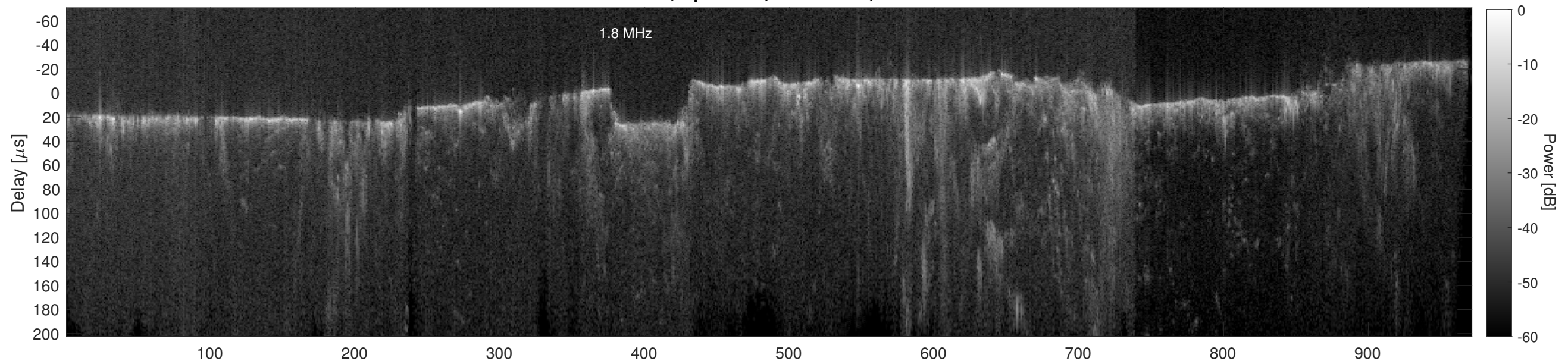
Orbit 11266, Cluttergram
