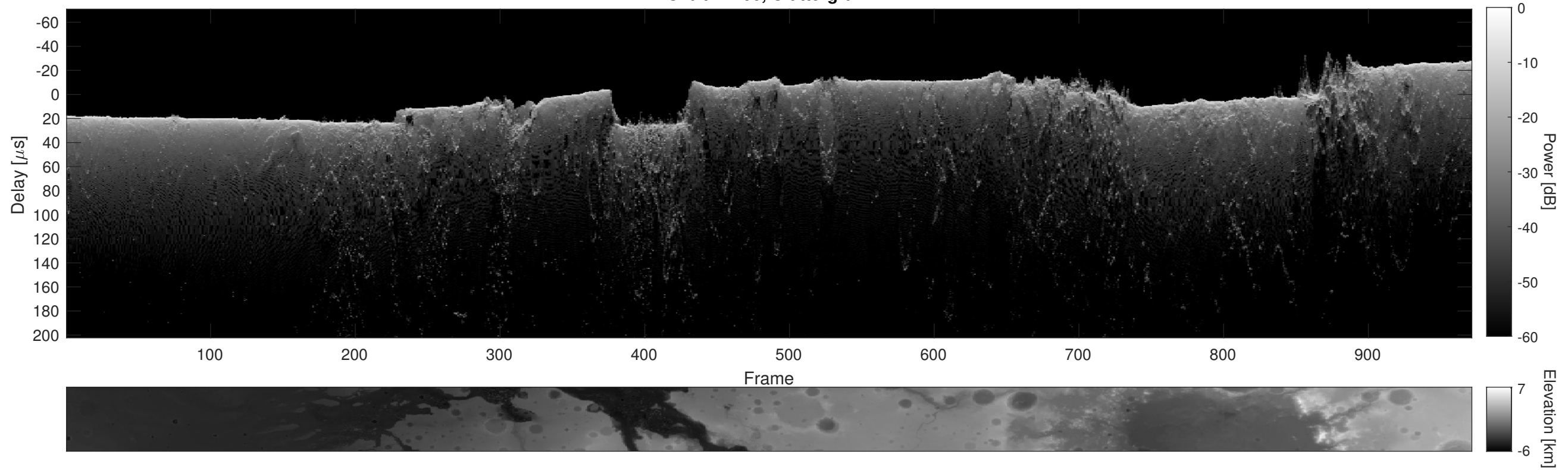
Orbit 11266, Cluttergram
