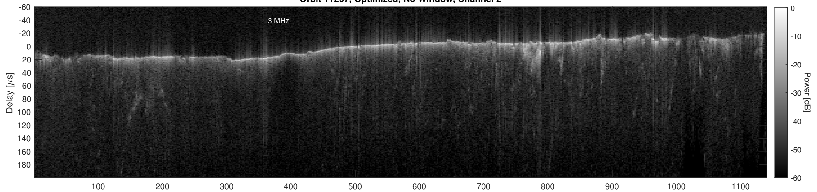
Orbit 11267, Cluttergram
