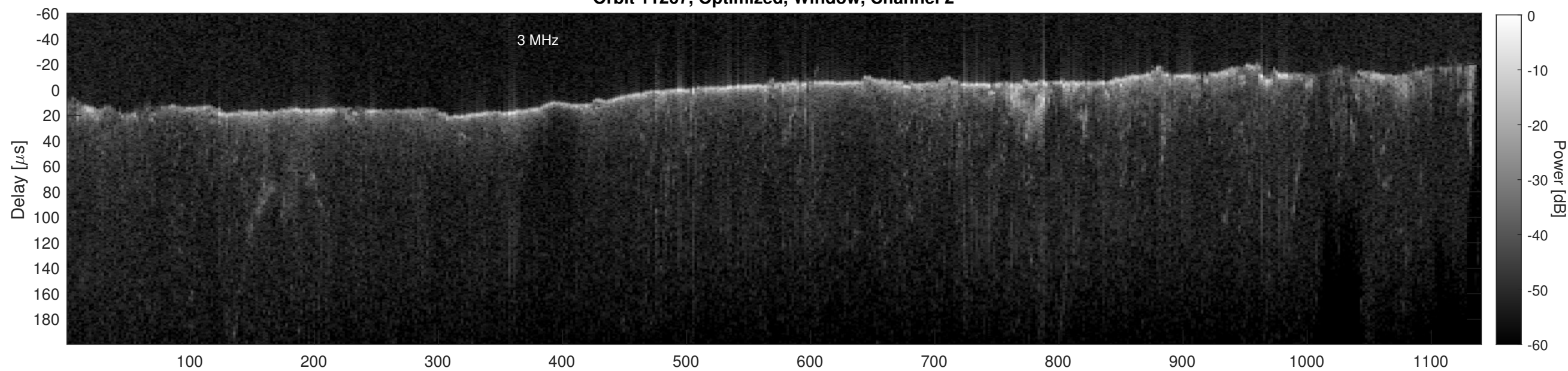
Orbit 11267, Cluttergram
