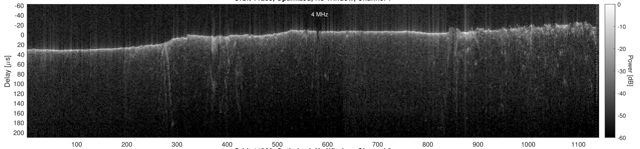
Orbit 11268, Optimized, No Window, Channel 2
