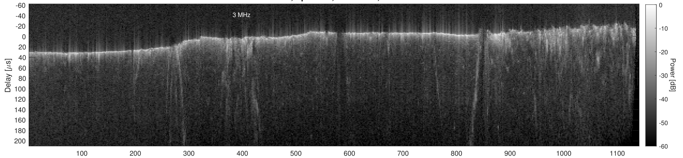
Orbit 11268, Cluttergram
