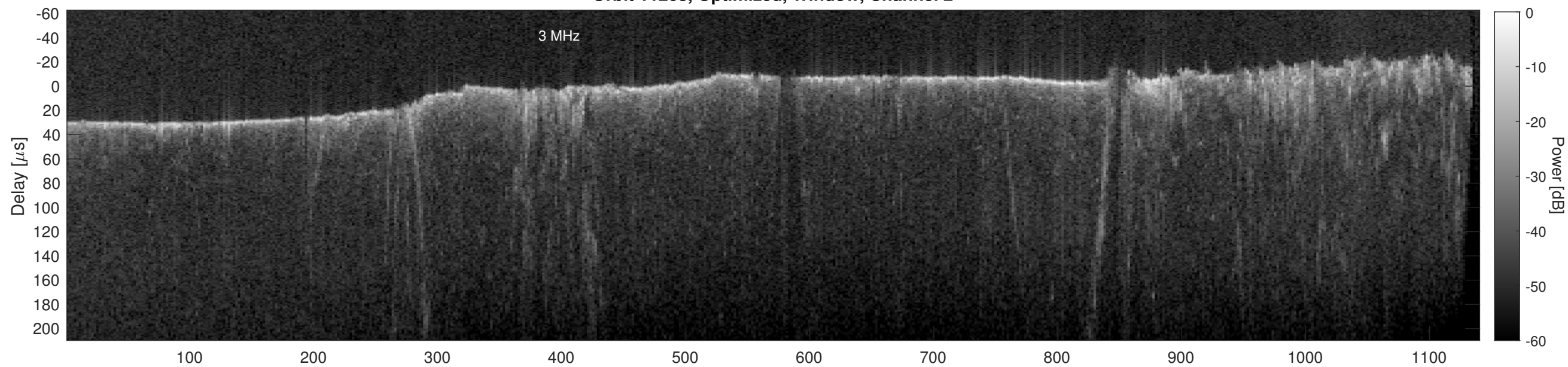
Orbit 11268, Cluttergram
