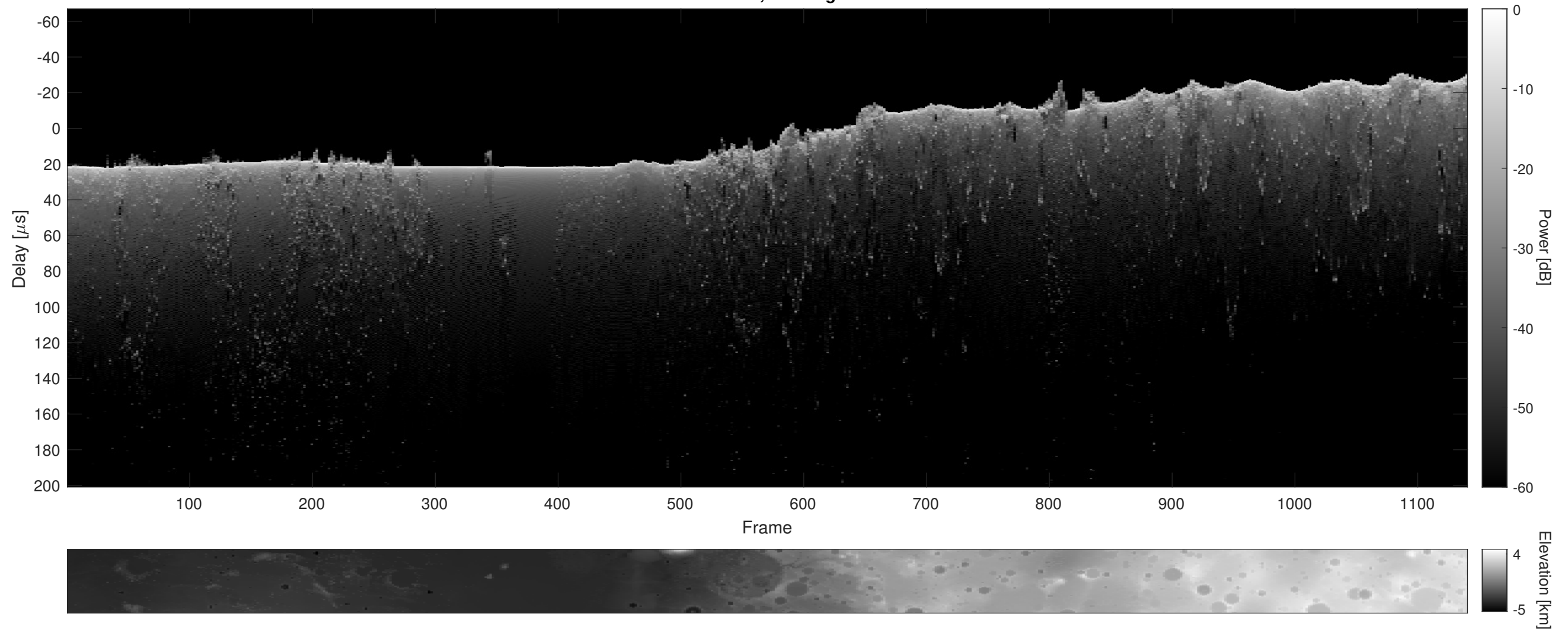
Orbit 11271, Cluttergram
