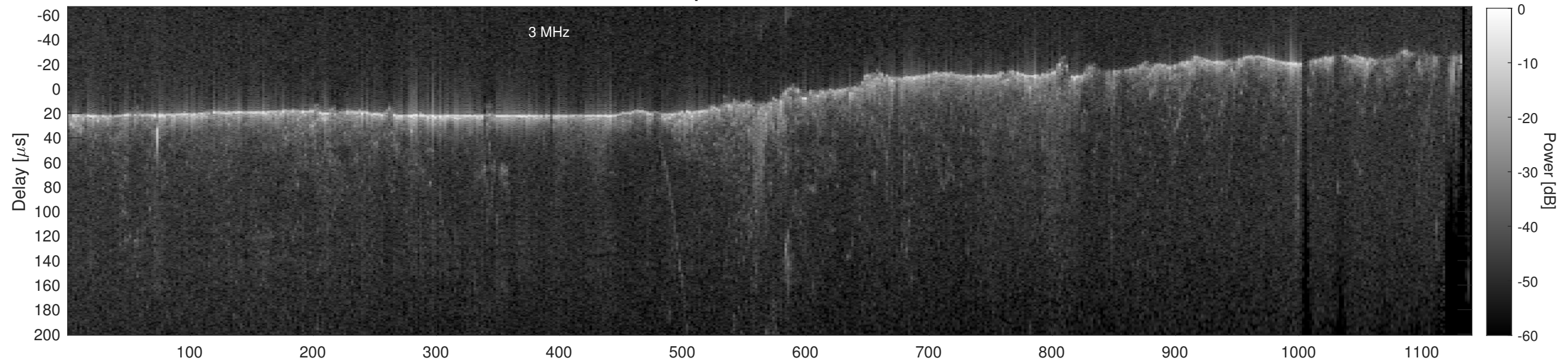
Orbit 11271, Cluttergram
