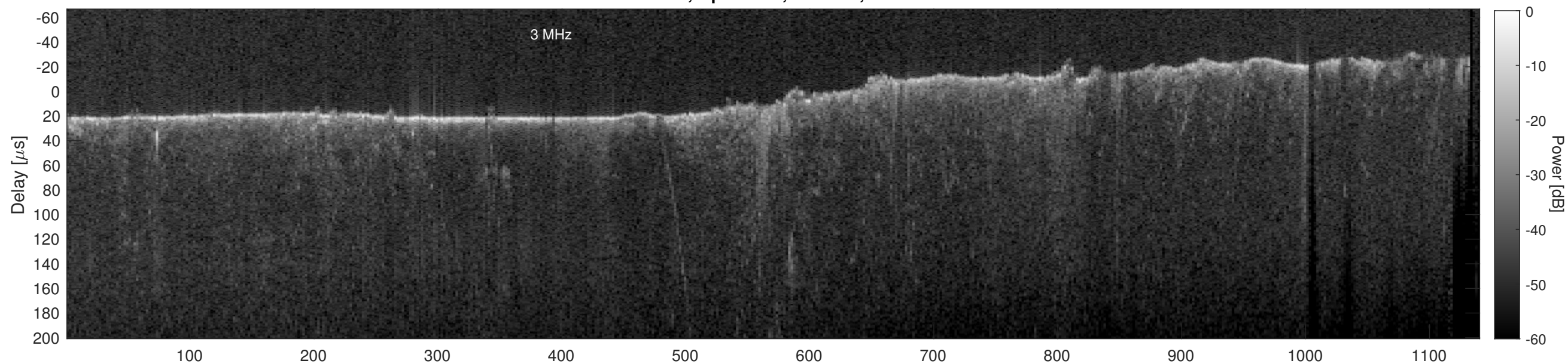
Orbit 11271, Cluttergram
