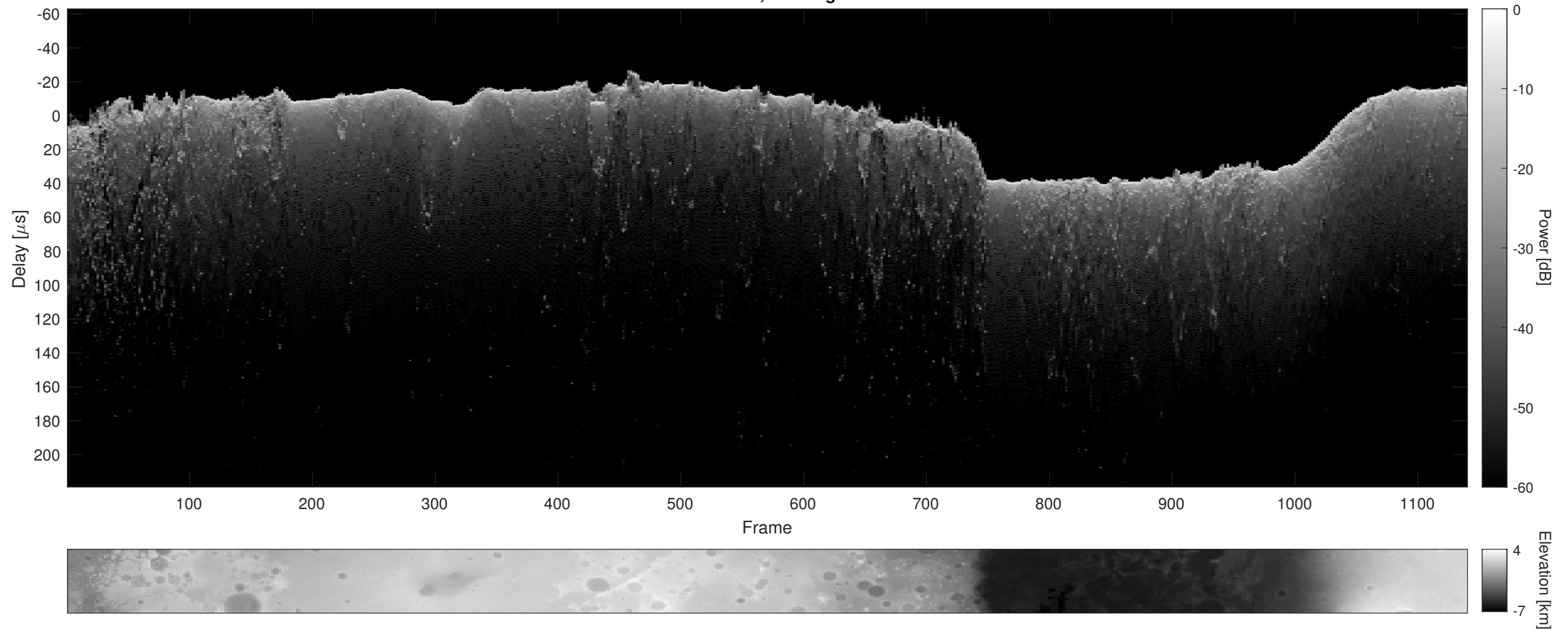
Orbit 11272, Cluttergram
