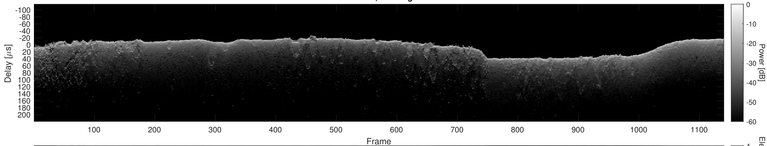
Orbit 11272, Cluttergram
