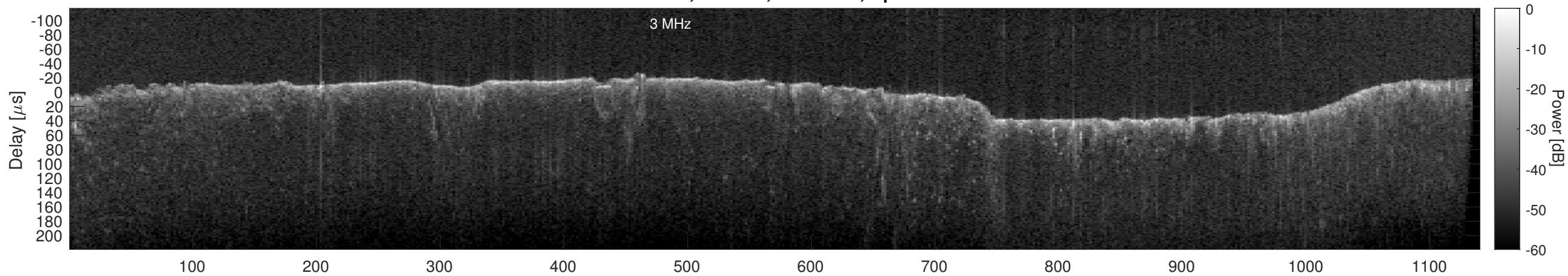
Orbit 11272, Cluttergram
