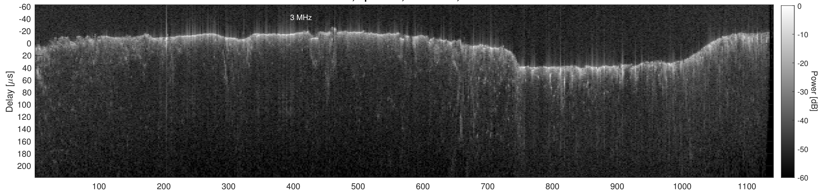
Orbit 11272, Cluttergram
