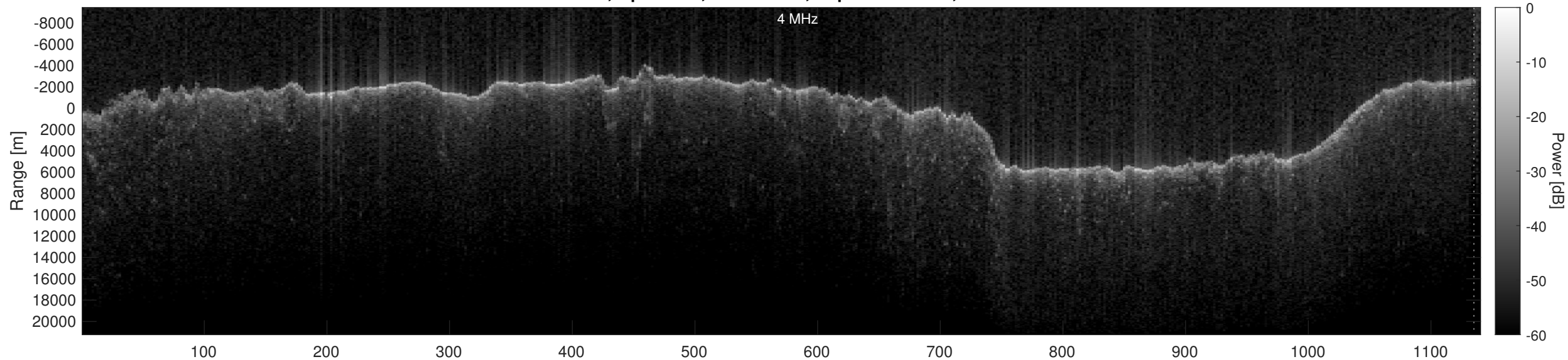
Orbit 11272, Optimized, No Window, Depth-Corrected, Channel 2
