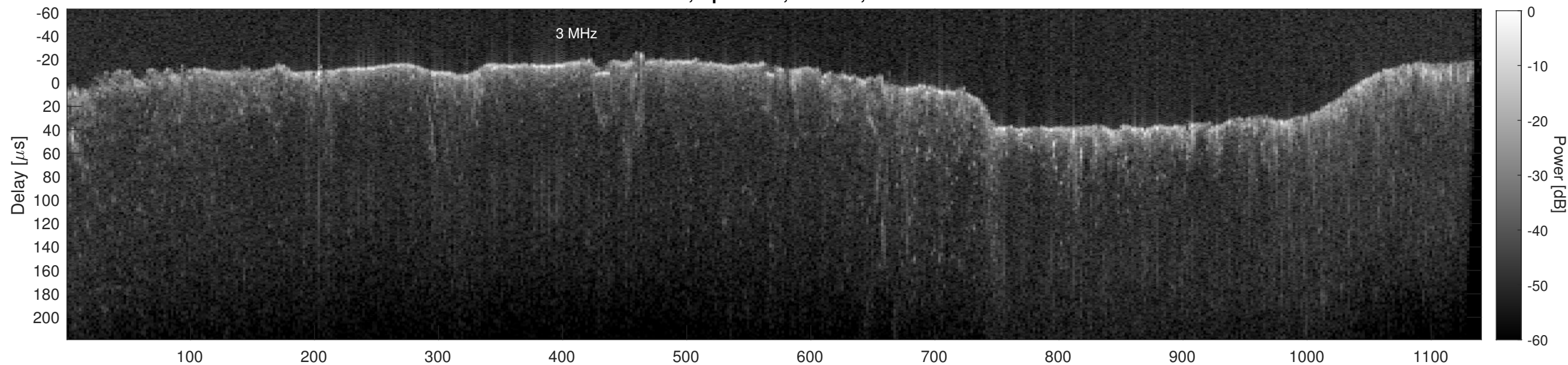
Orbit 11272, Cluttergram
