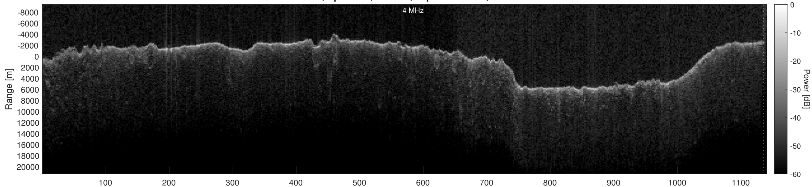
Orbit 11272, Optimized, Window, Depth-Corrected, Channel 2
