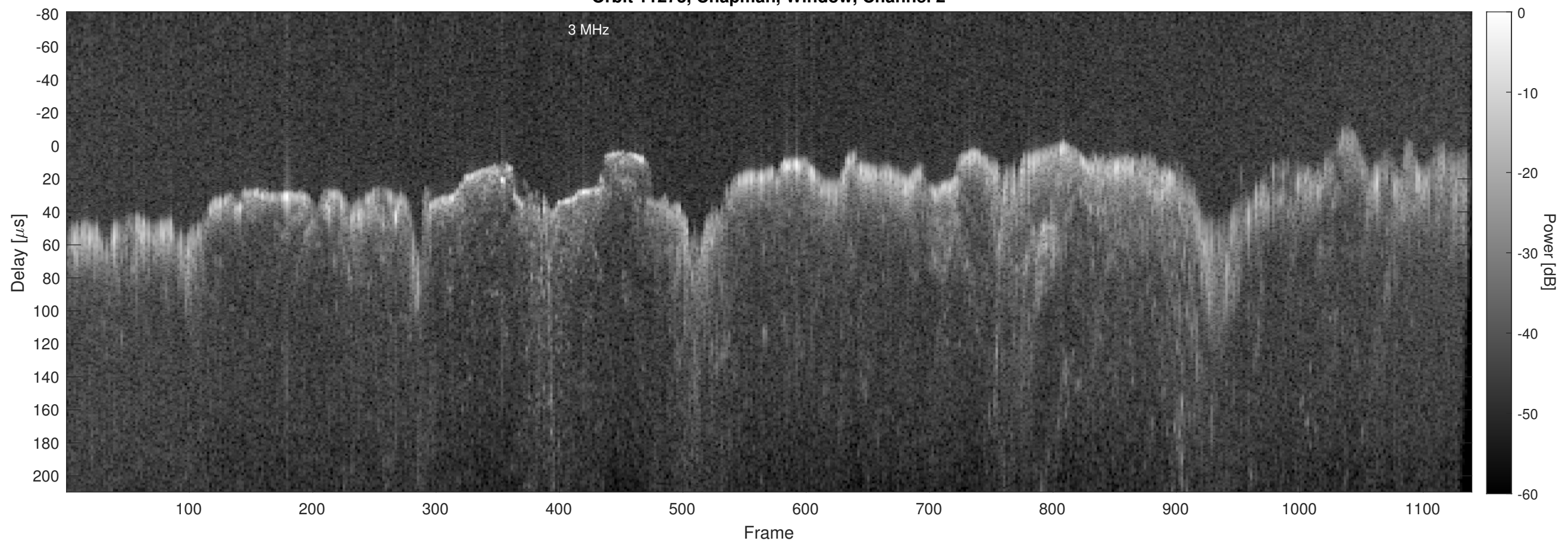
Orbit 11273, Chapman, Window, Channel 2
