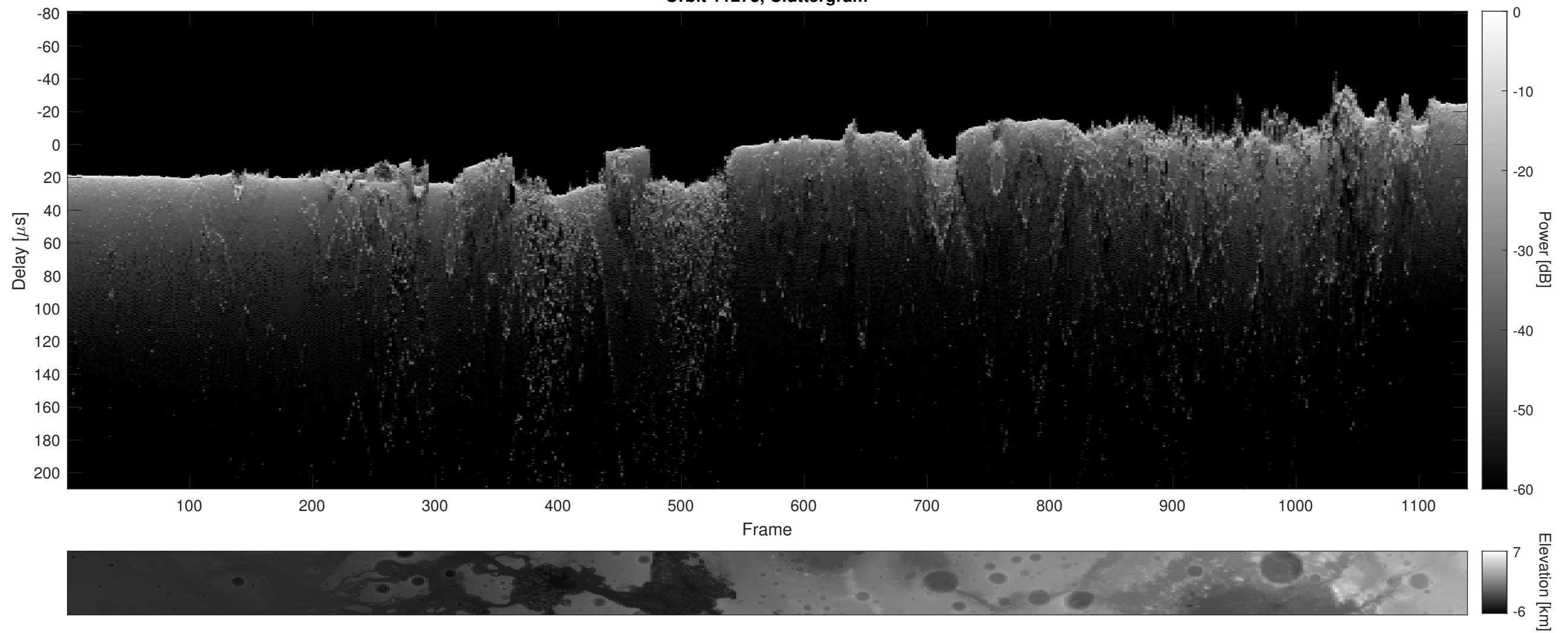
Orbit 11273, Cluttergram
