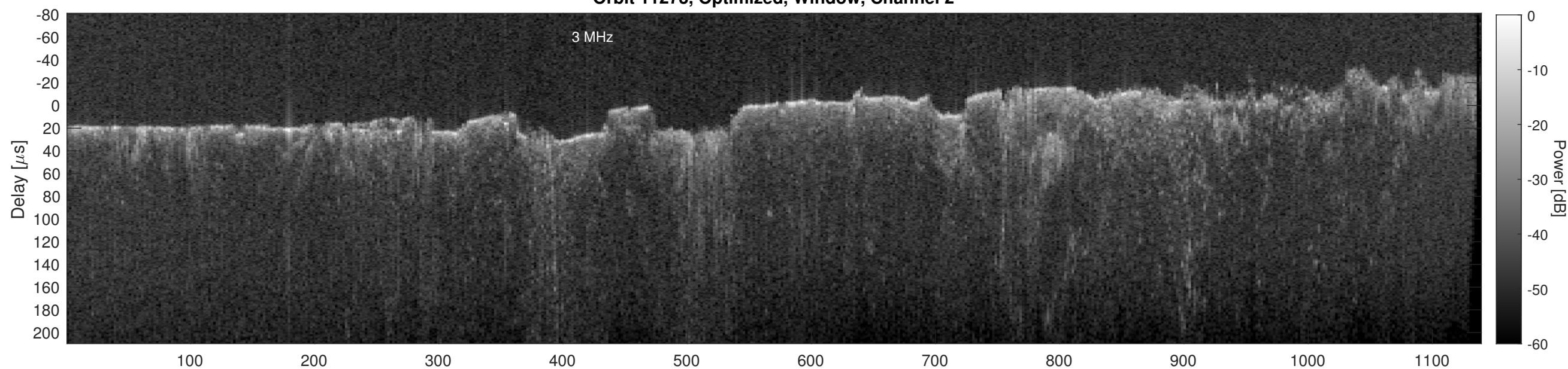
Orbit 11273, Cluttergram
