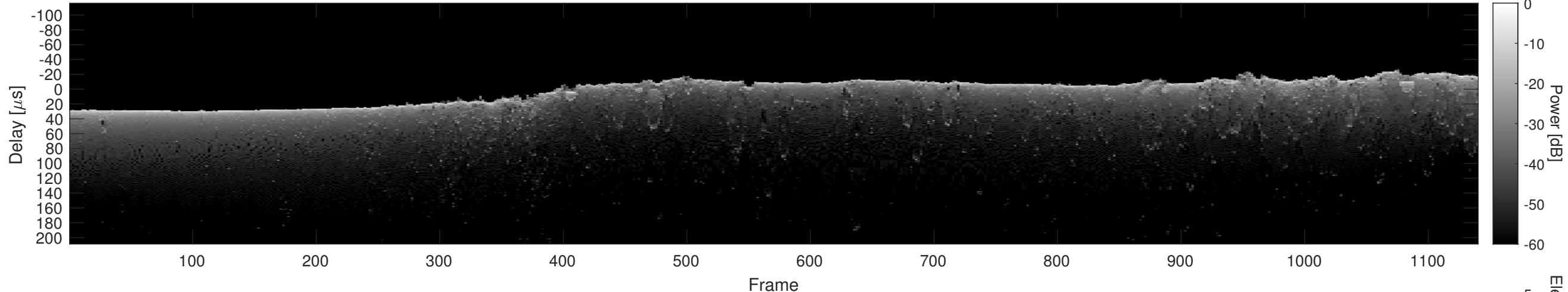
Orbit 11275, Cluttergram
