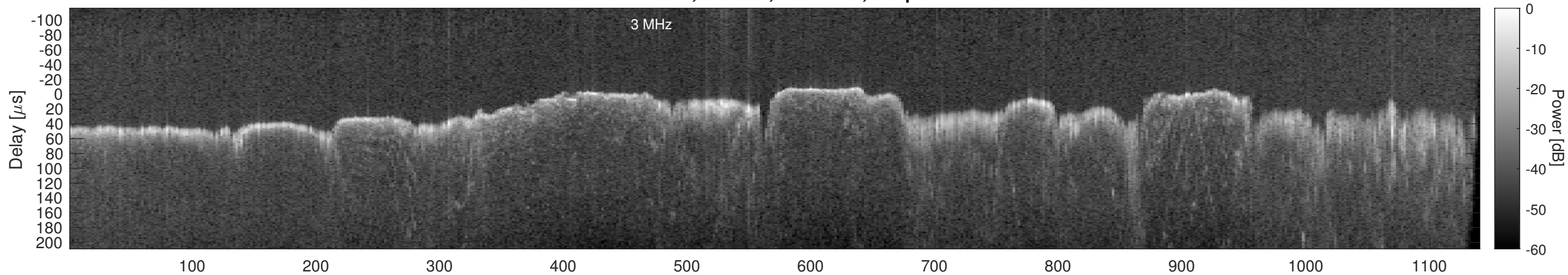
Orbit 11275, Window, Channel 2, Optimized
