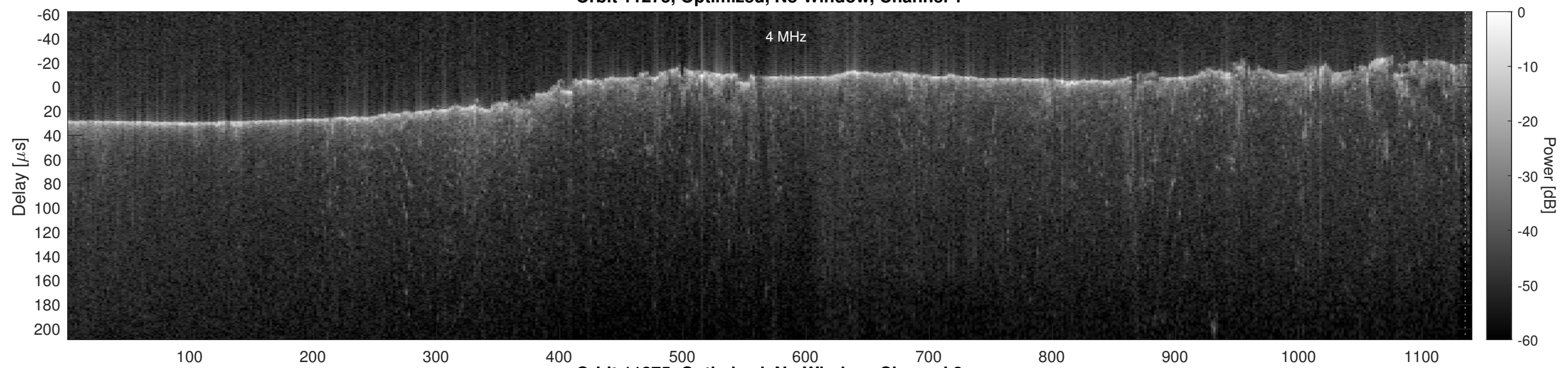
Orbit 11275, Optimized, No Window, Channel 2
