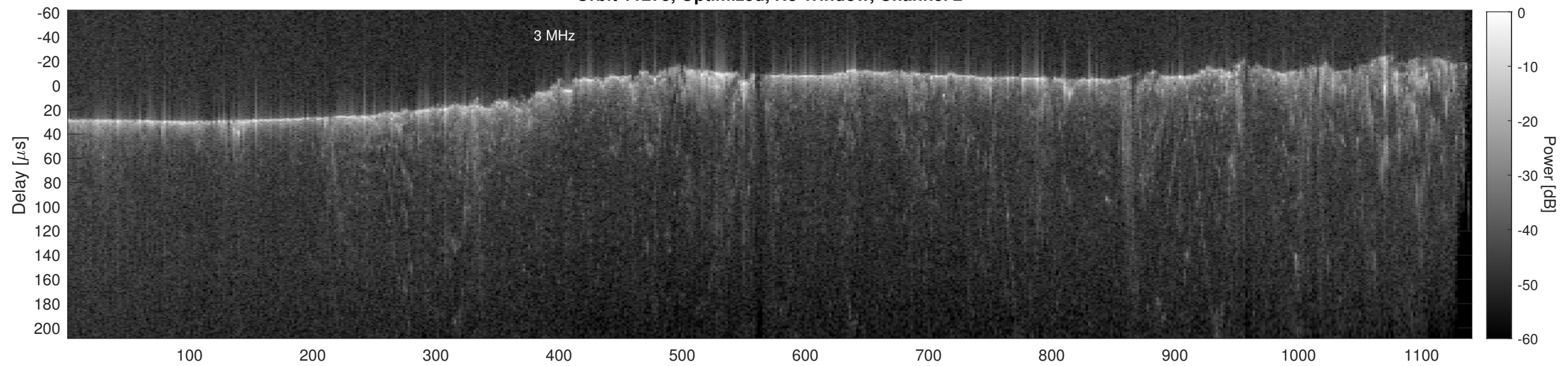
Orbit 11275, Cluttergram
