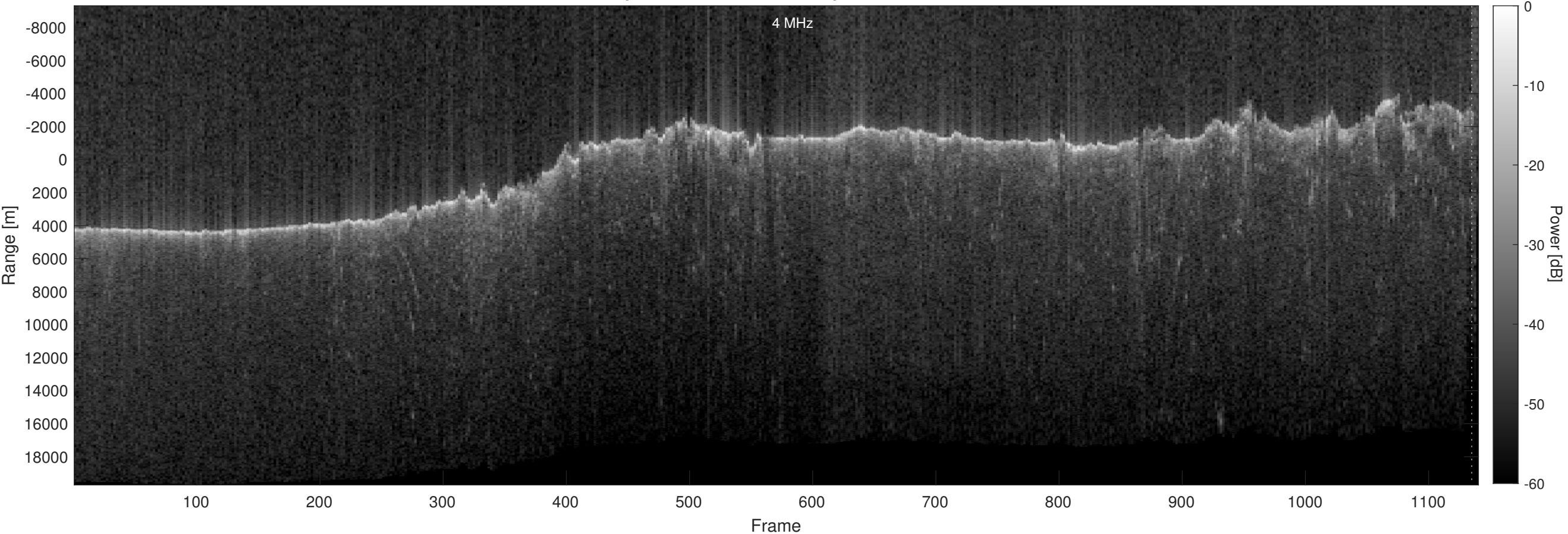
Orbit 11275, Optimized, No Window, Depth-Corrected, Channel 2
