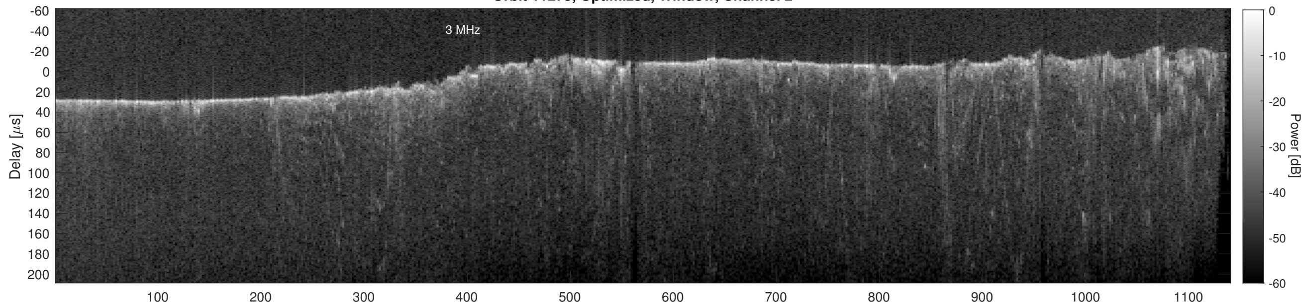
Orbit 11275, Cluttergram
