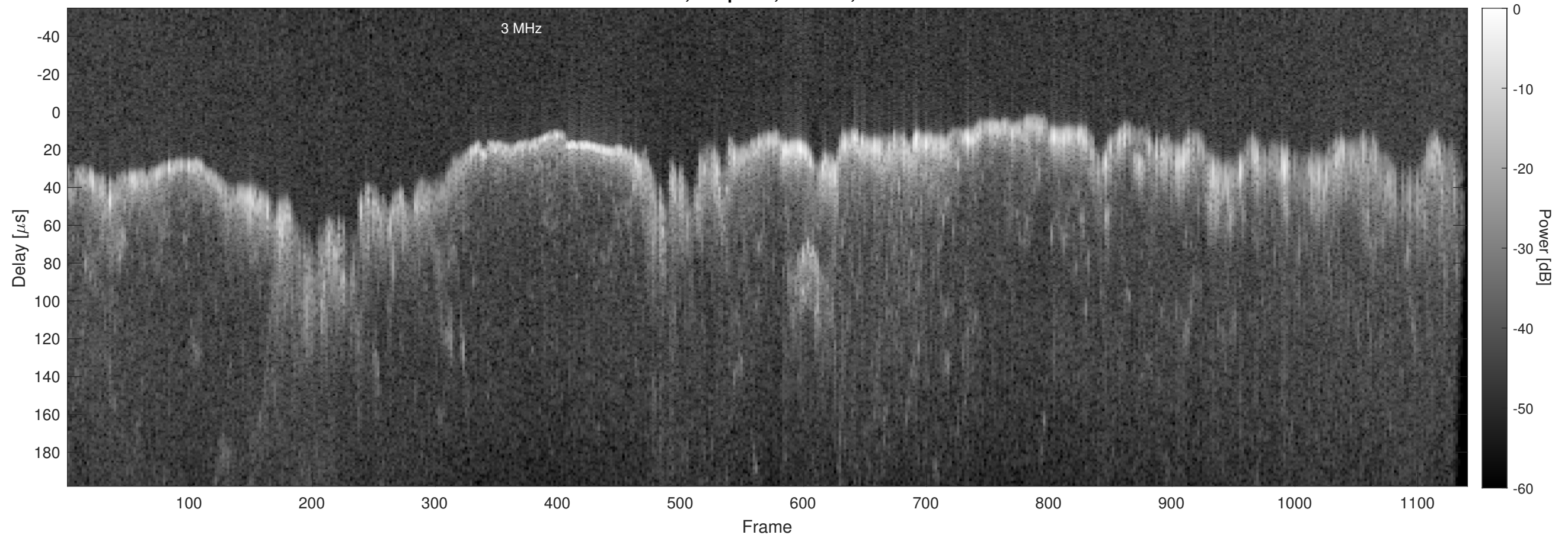
Orbit 11276, Chapman, Window, Channel 2
