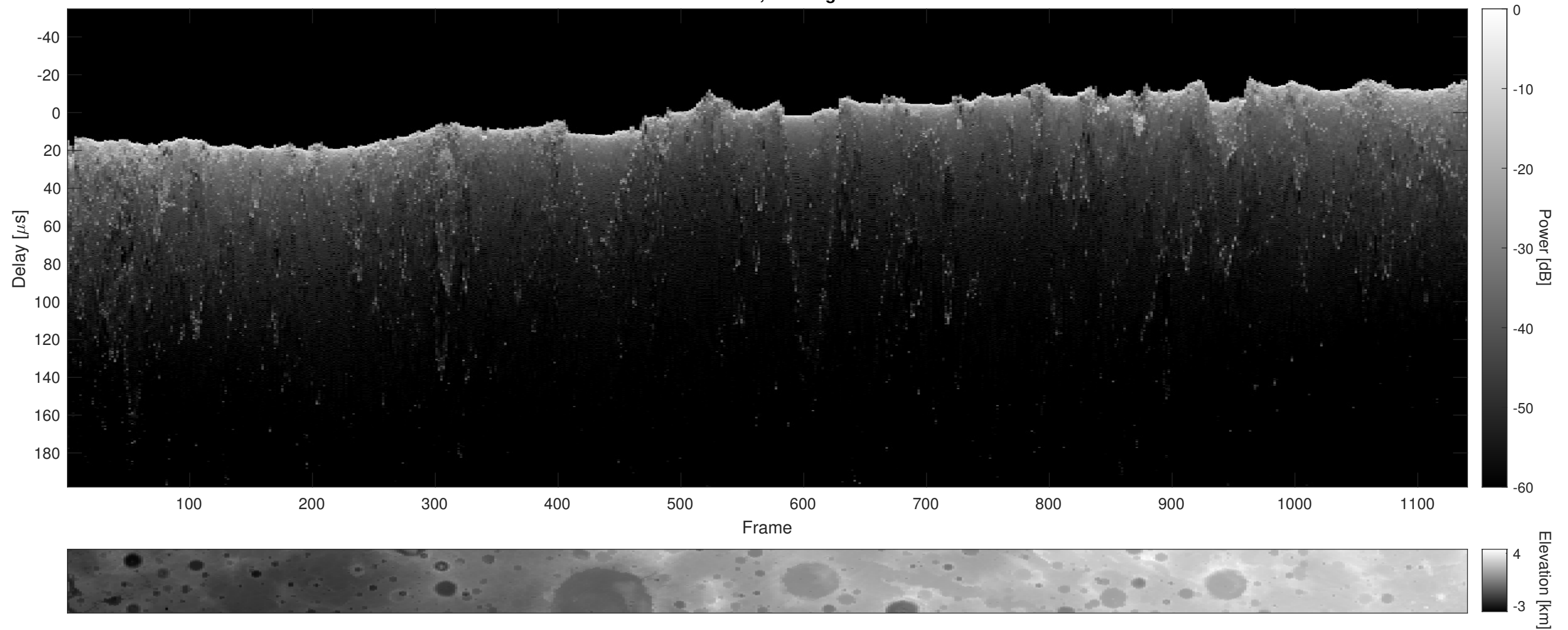
Orbit 11276, Cluttergram
